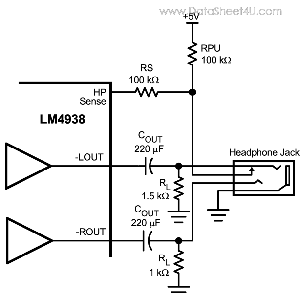
FIGURE 3. Headphone Sensing Circuit
